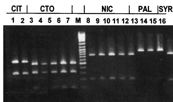
Figure 2. HaeIII digestion of PCR products amplified with primers ITS4 and ITS6. Lanes 1–2: DNA from P. citricola 61 and 277; lanes 3–7: DNA from P. citrophthora 112, 114, 155, 163 and 244; M: 123 bp ladder; lanes 8–12: DNA from P. nicotianae 44, 113, 115, 219 and 220; lanes 13–15: DNA from P. palmivora 292, 296 and 178; lane 16: DNA from P. syringae 513.
